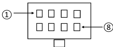
Connector (Front View) Molex 39-01-2085 (Pins: Molex 39-00-0208)
